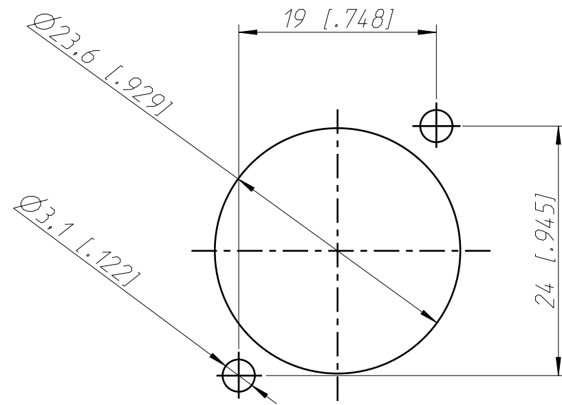
panel cut out (rear side)
