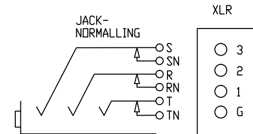
NORMALLING-SCHEMES
