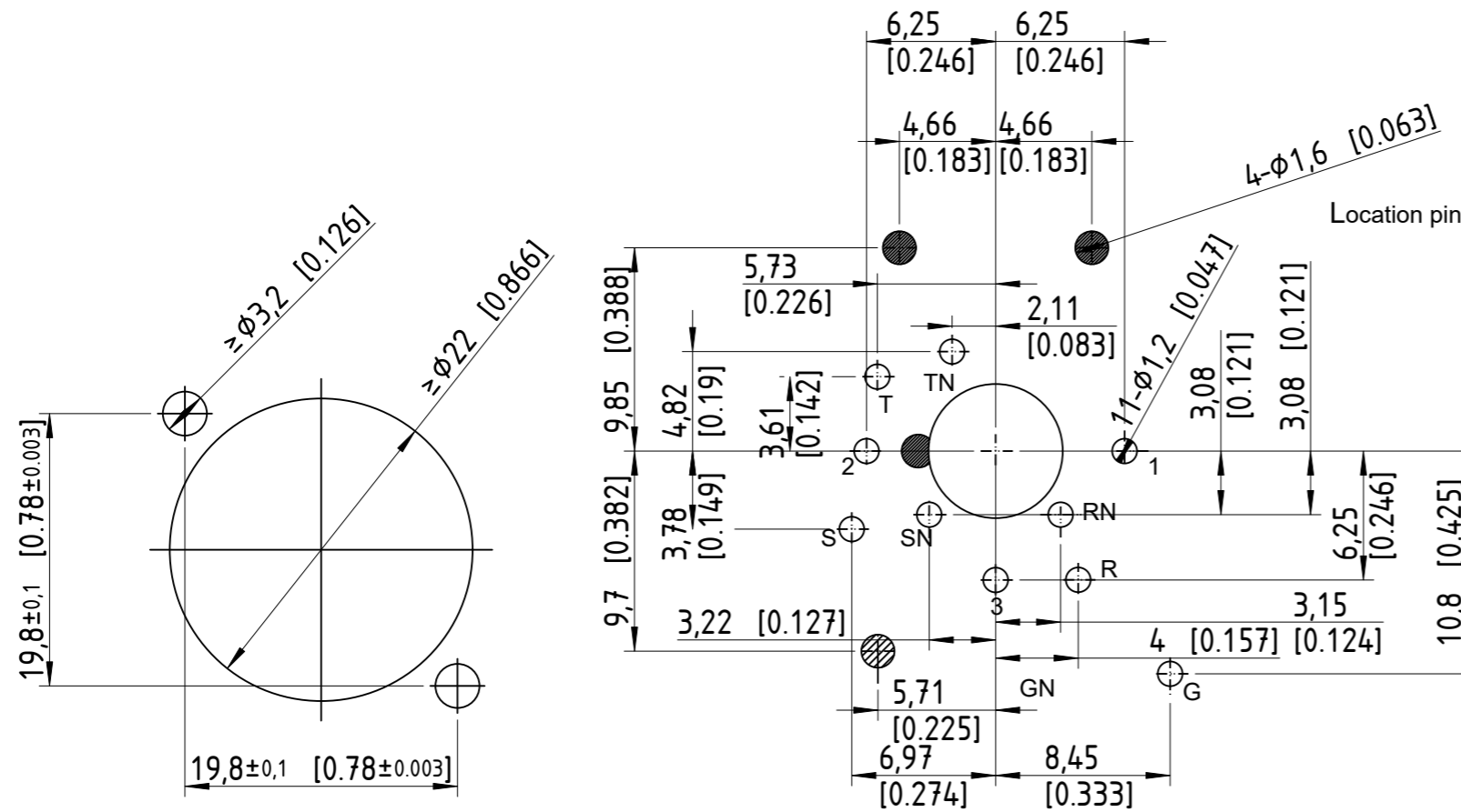
PCB Layout(Component side) tolerance ±0.05 [0.002]
