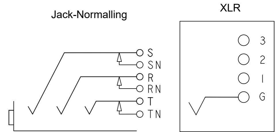
Normalling-Schemes
